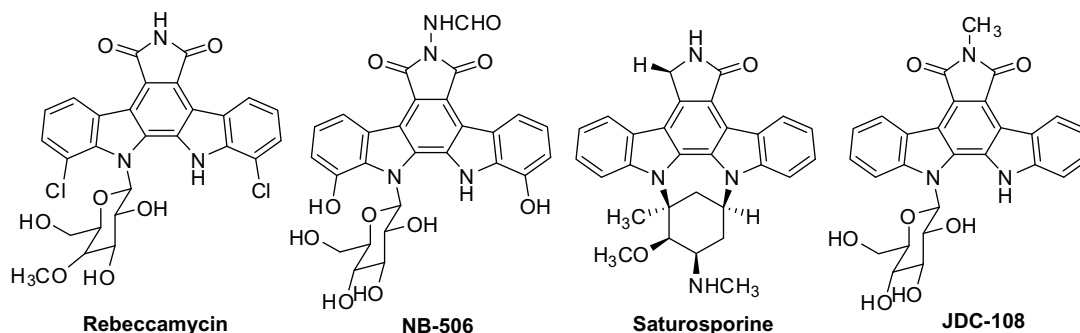
Figure 1. Structure of the mentioned indolocarbazole derivatives.
