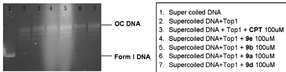
Figure 2. The effect of 9a , 9b , 9d , and 9e on DNA-TOPO I complex.
